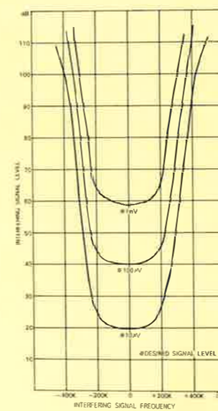
SELECTIVITY
