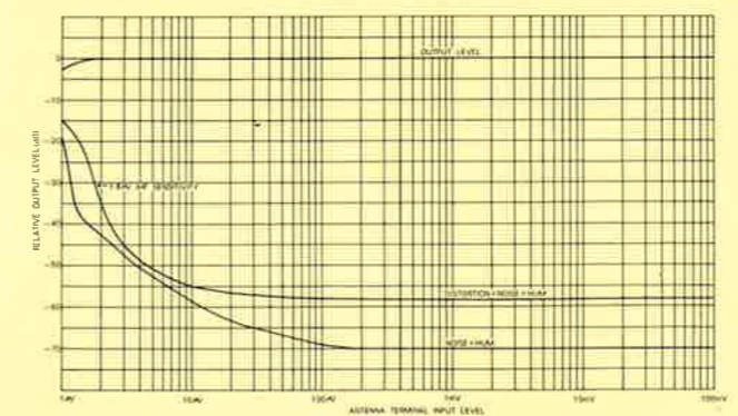
FM CHARACTERISTIC
